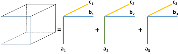
Fig. 2: Schematic of tensor of rank three.
